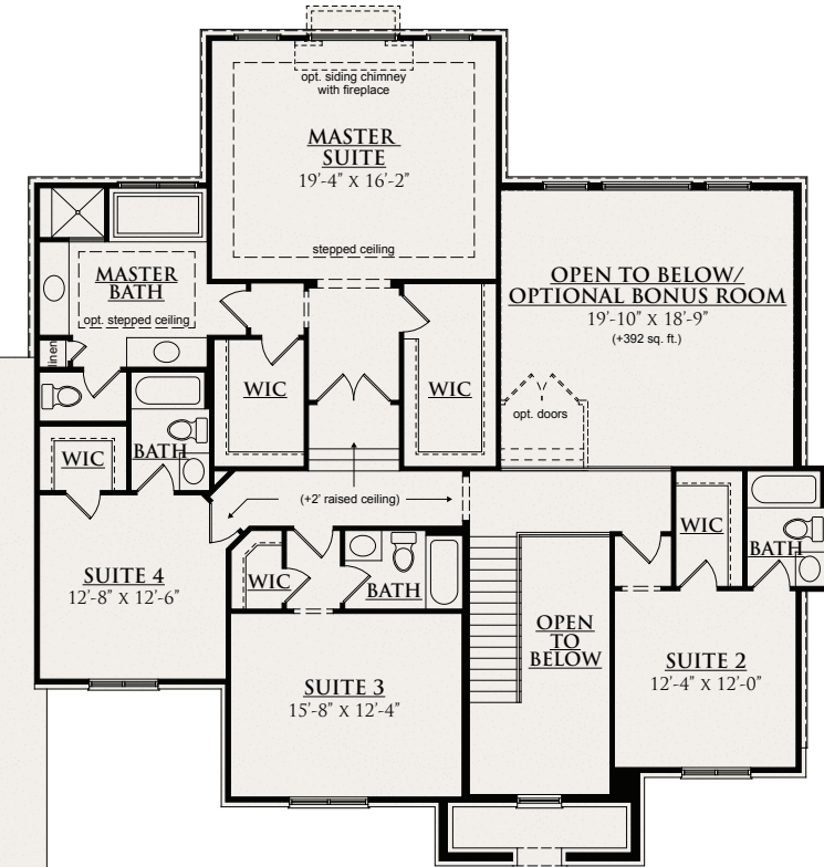
SECOND FLOOR
